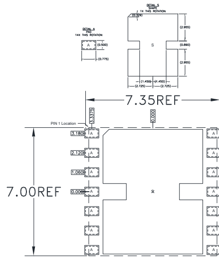
RECOMMENDED LAND PATTERN MASK
