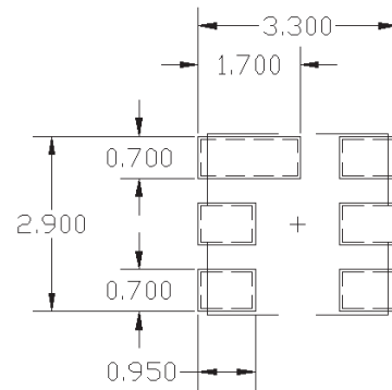
Top view recommended land pattern stencil aperture.
