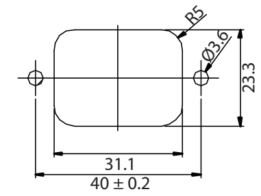
PANEL CUTOUT
