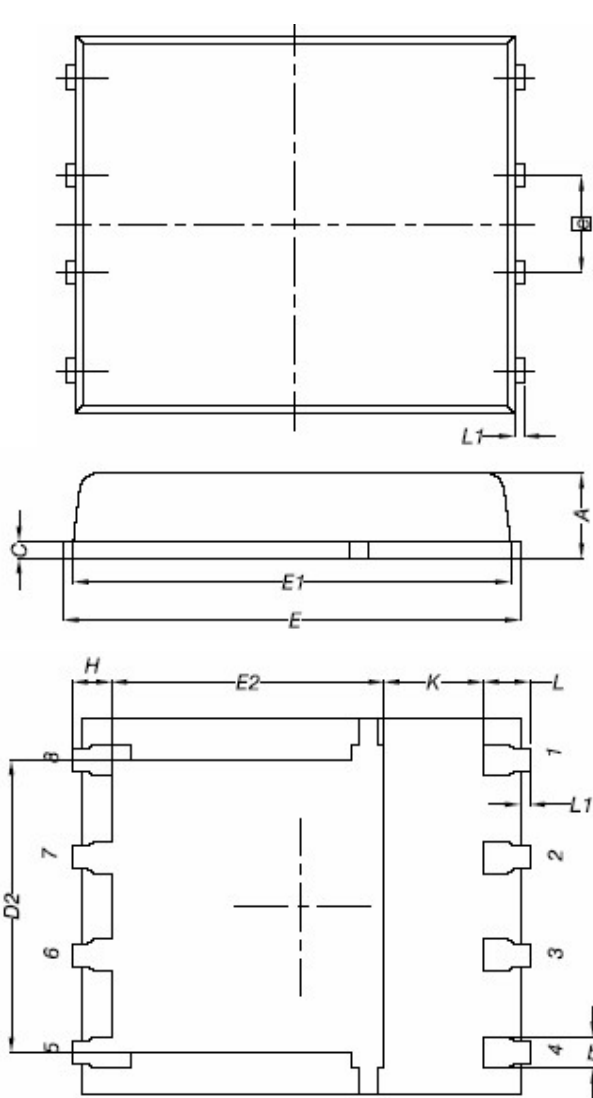
BACKSIDE VIEW
