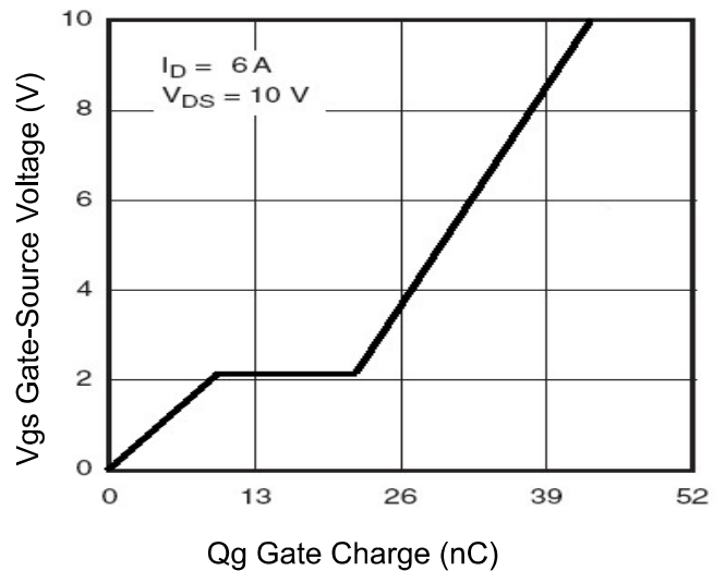
Figure 4 Gate Charge
