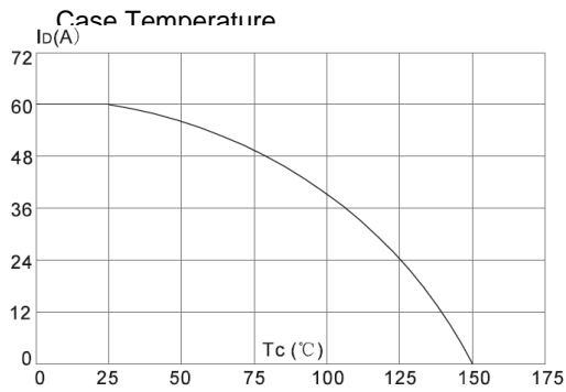
Figure 9: Maximum Drain Current vs. Case Temperature
