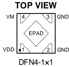
Figure 2. Pin Configuration
