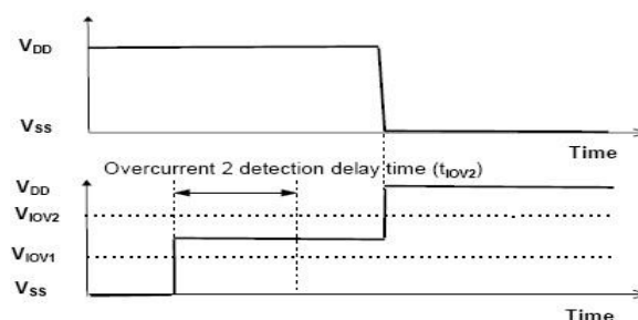
Figure 4. Overcurrent delay time
