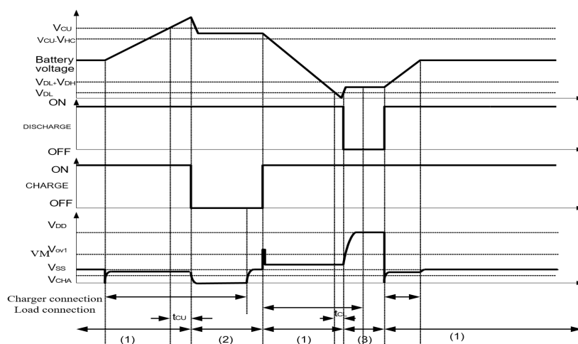
Figure5-1 Overcharge and Overdischarge Voltage Detection
