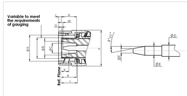
CEI Dimensions (in mm)
