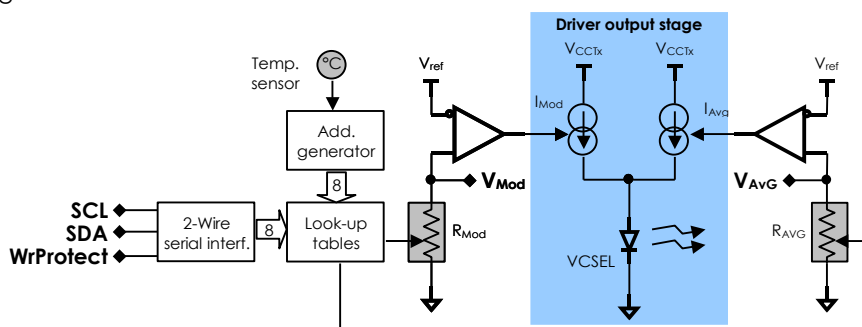
Figure 6 - Average and modulation current control circuit
