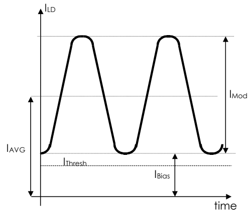
(b) Laser diode currents
