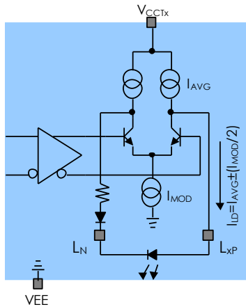
(a) Output stage
