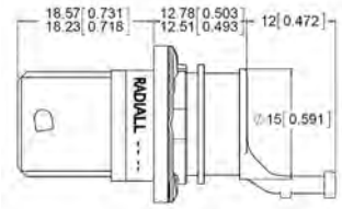
Rear output #A Banding platform and tie-wrap
