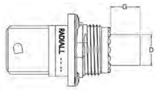
Rear output #2 Accessory Thread
