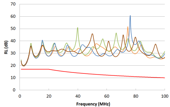
Return Loss (RL):
