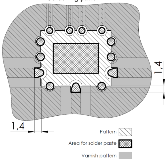
Soldering pattern
