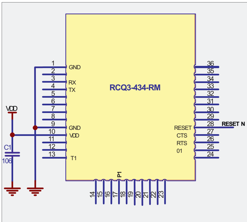
Reference Schematics
