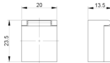
Dimensioned drawing
