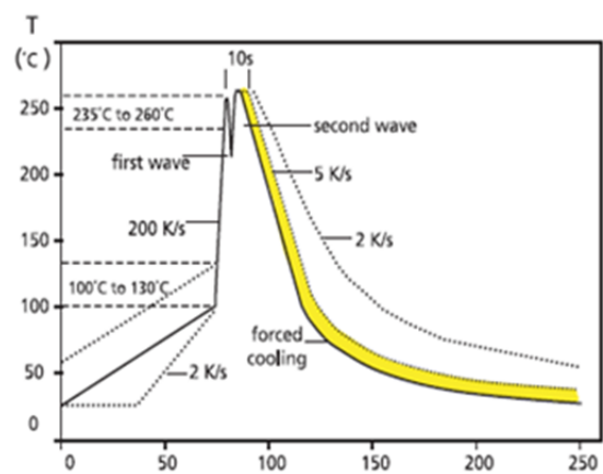
Recommended double-wave Soldering Profile
