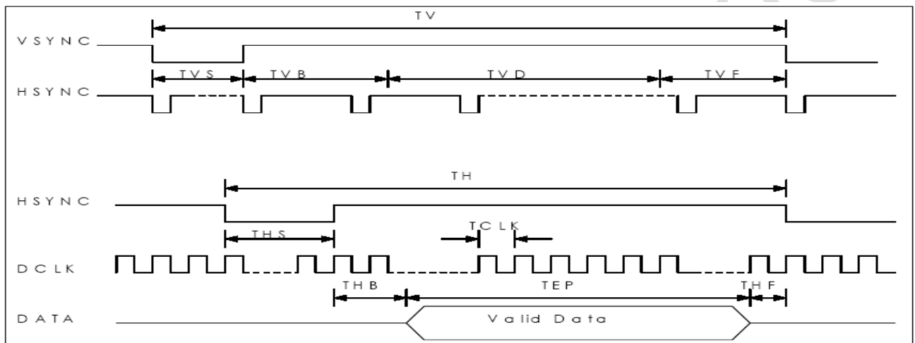
Figure 7.2.1 IHS and IVS timing waveforms
