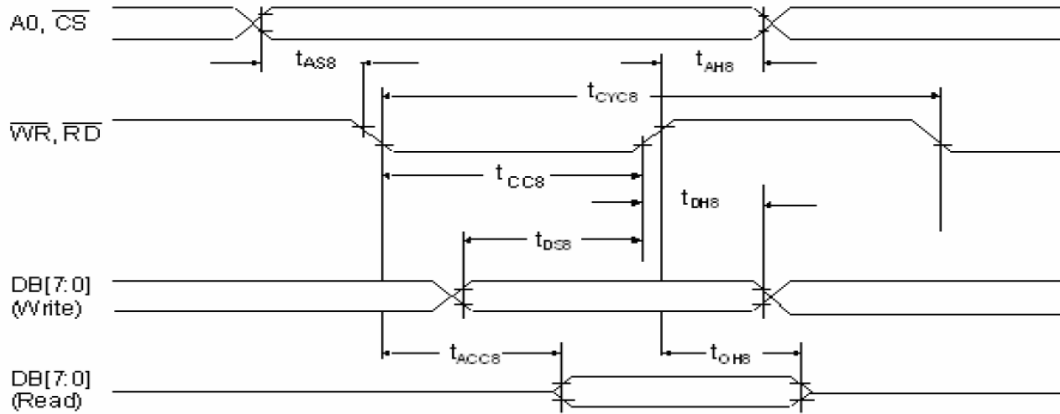
Figure 2: 8080 Waveform Table 2: 8080 MCU I/F Timing
