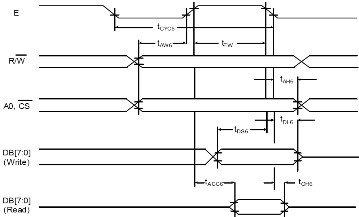
Figure 1: 6800 MCU Waveform
