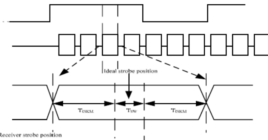
LVDS timing(3)
