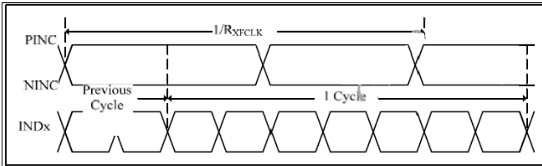
LVDS timing(1)
