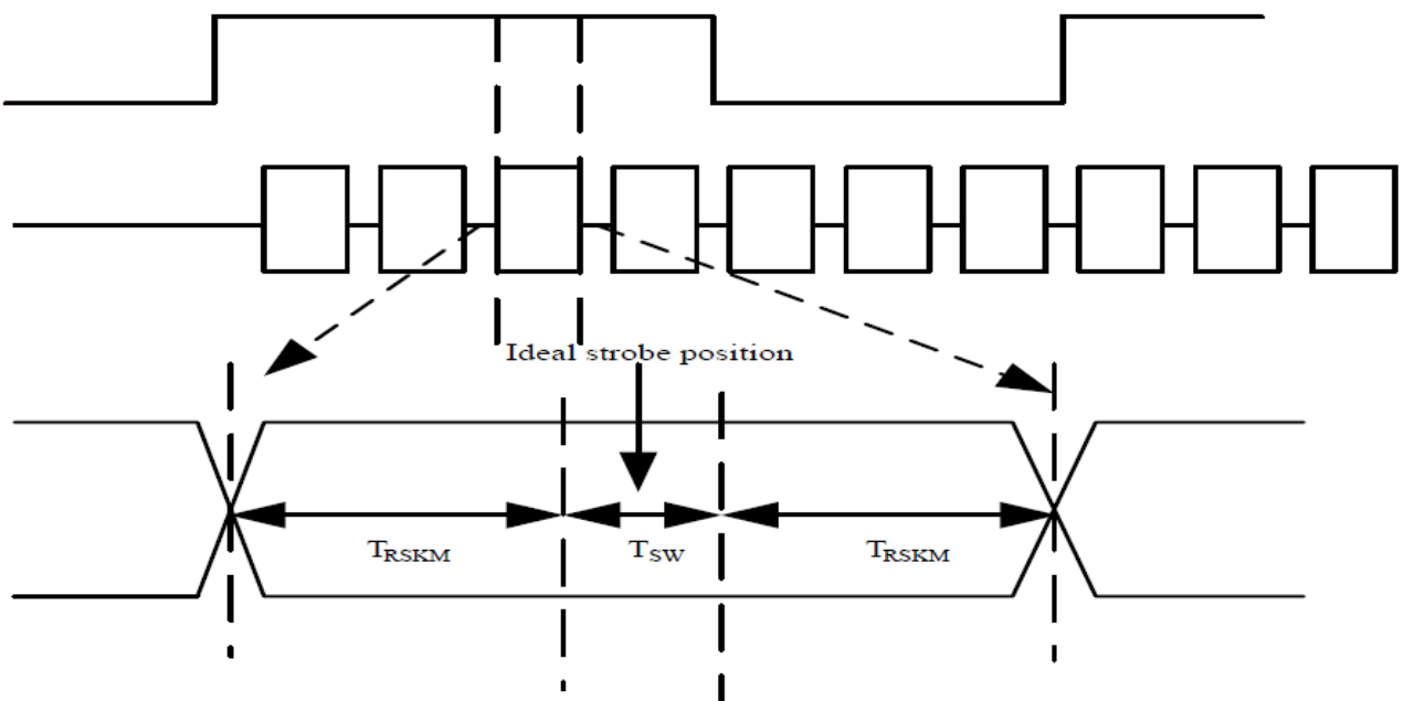
LVDS timing(2)
