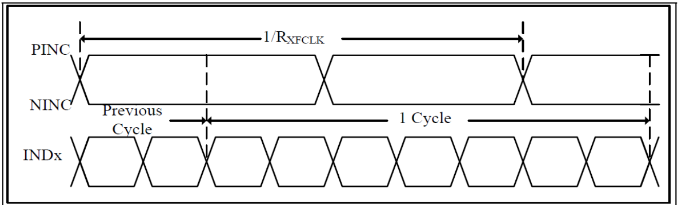
LVDS timing(1)
