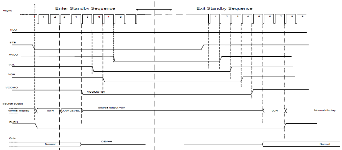
Enter and Exit Standby Mode timing chart
