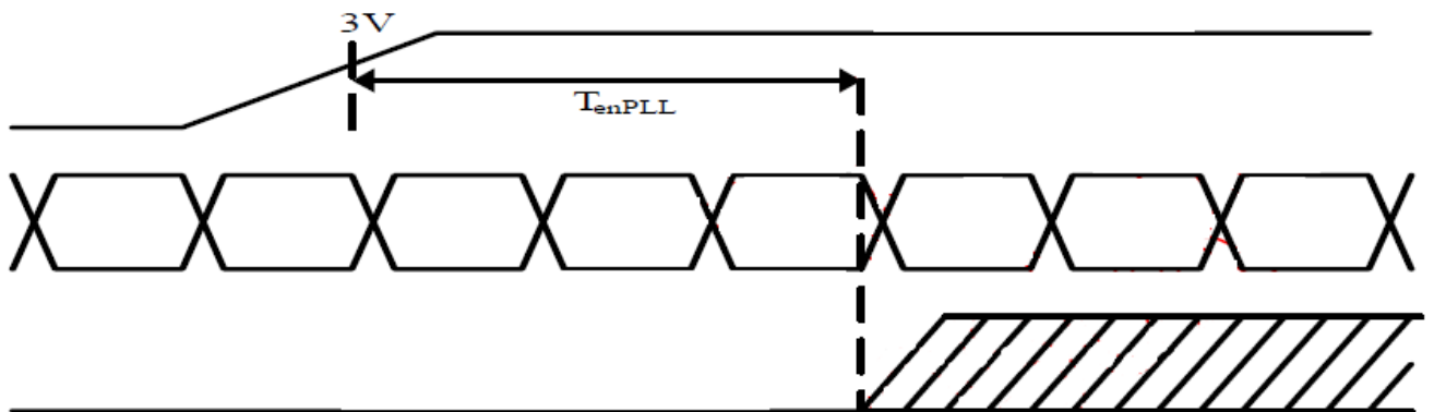
LVDS timing(2)
