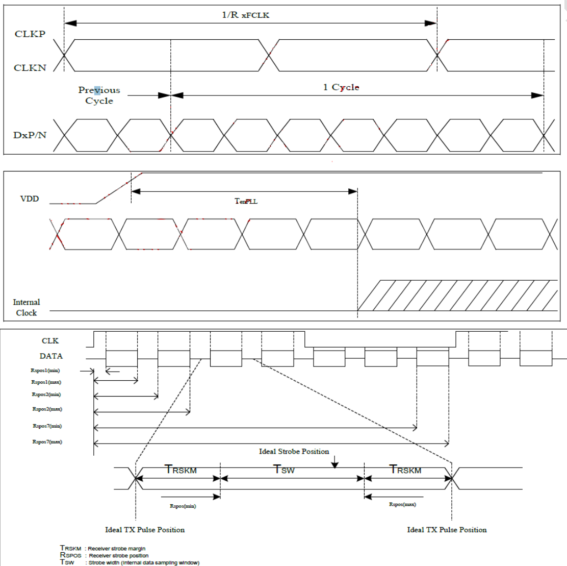
Figure 1: LVDS figure
