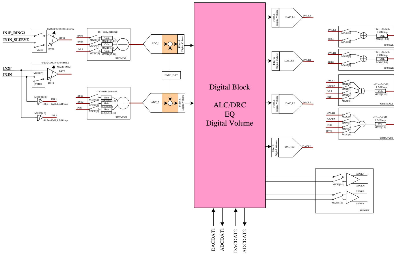
Figure 2. Audio Mixer Path
