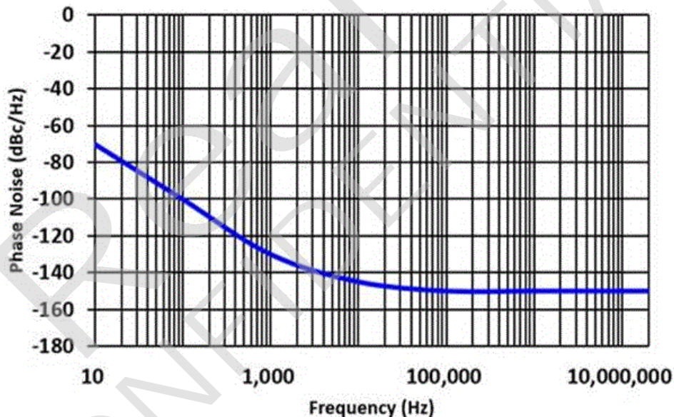
Figure 7. Phase Noise
