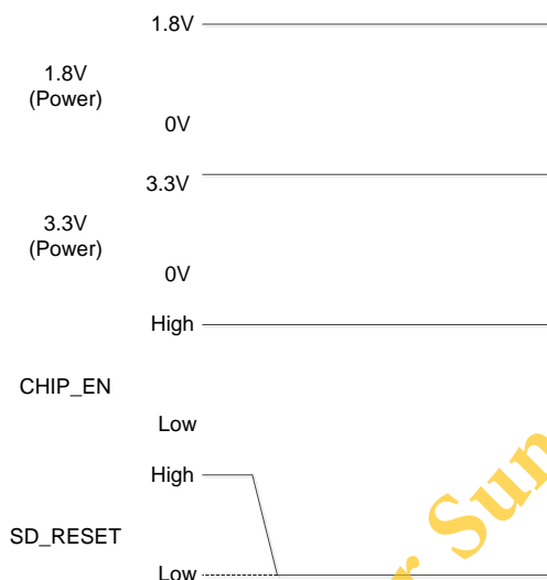
Figure 7. WLAN and SDIO/G-SPI Power Off Sequence
