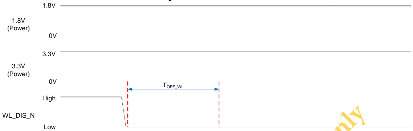
Figure 9. WLAN Radio Off Sequence
