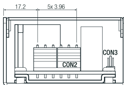
DC side
