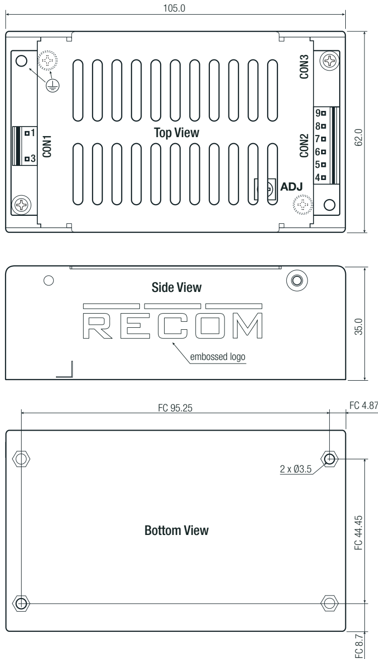
DC side
