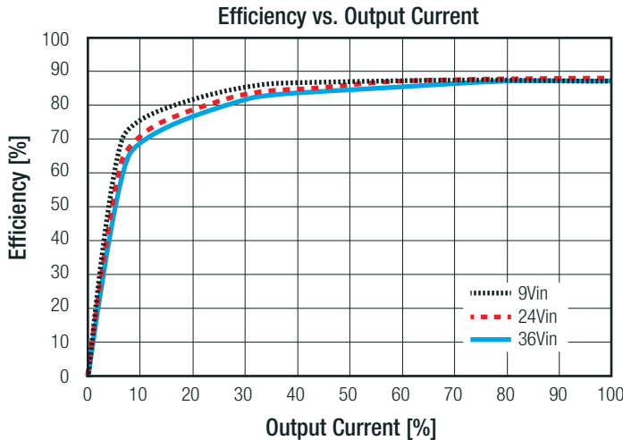
RPA20-2412DAW
