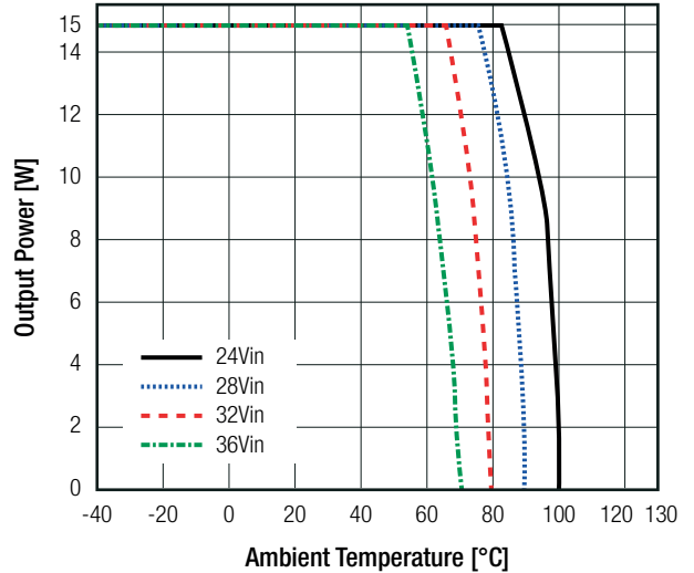
Thermal Derating
