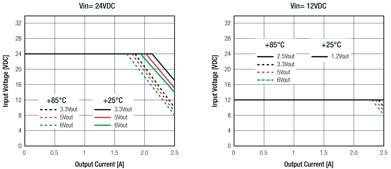
Input voltage vs. output current (tested without additional test PCB)
