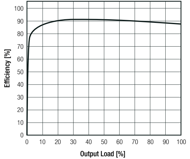
V_{\text{out}} = 5\text{VDC} , V_{\text{in}} = 24\text{VDC} (2.1A max.)
