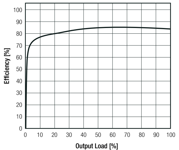
V_{\text{out}} = 5\text{VDC} , V_{\text{in}} = 24\text{VDC} (2.1A max.)
