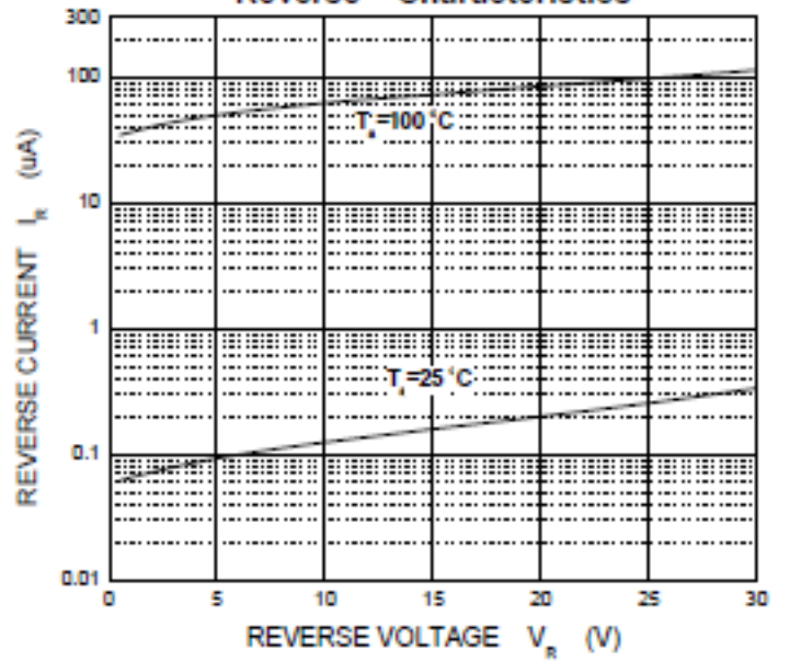
Reverse Characteristics
