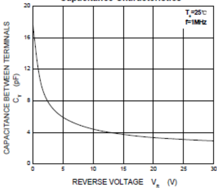
Capacitance Characteristics
