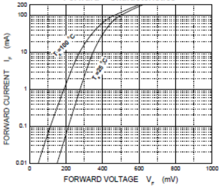
Forward Characteristics
