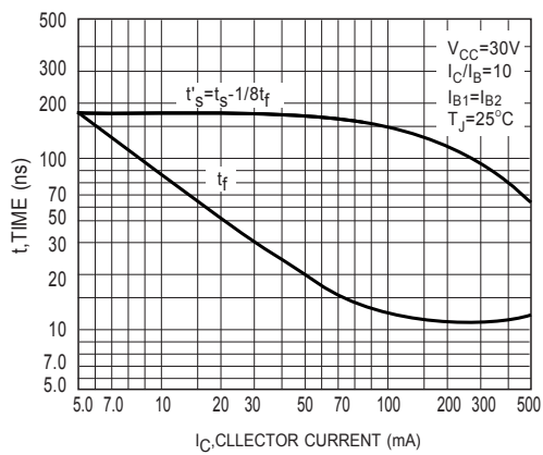
Figure 4. Turn-Off Time
