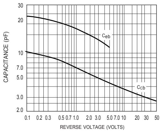
Figure 7. Capacitances
