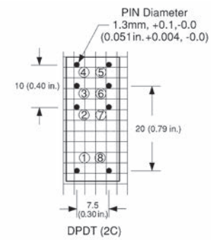
Bottom View, Relay Pinouts, Grid 2.54mm (0.1 in.)
