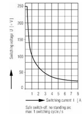
Maximum switching power curve
