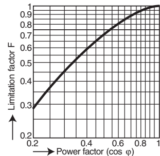
Limitation factor for inductive loads
