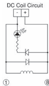
Bottom View, Relay Pinouts, Grid 2.54mm (0.1 in.)
