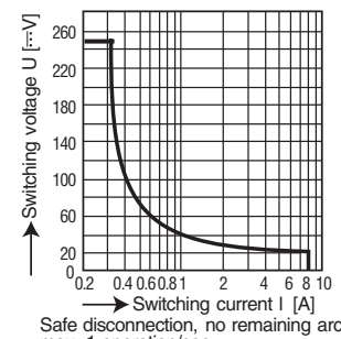
Maximum switching power curve Safe disconnection, no remaining arc, max. 1 operation/sec.
