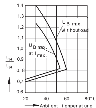
Relay operation voltage vs. ambient temperature
