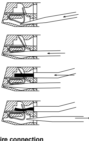
Wire connection
