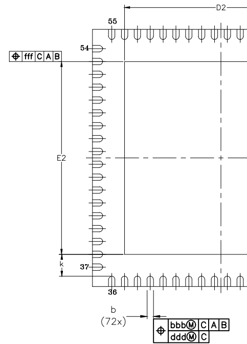
BOTTOM VIEW
