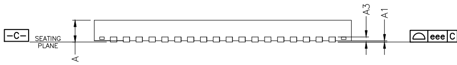
SIDE VIEW
