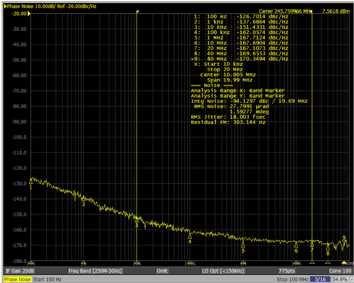
Figure 23. Phase Noise Performance of 245.76MHz Input Reference Clock
