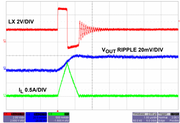
FIGURE 16. STEADY STATE OPERATION AT NO LOAD (PFM)
