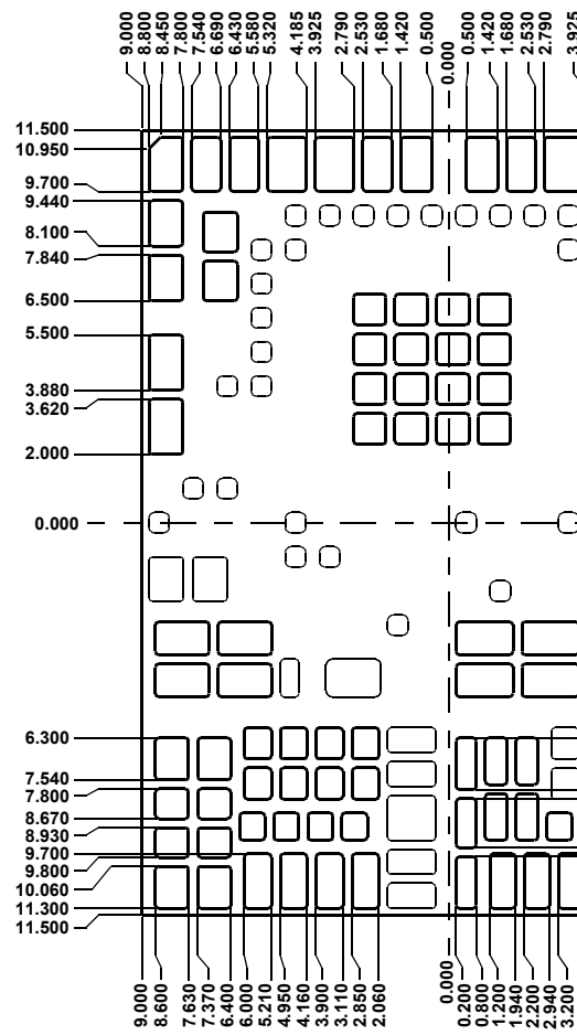
PCB LAND PATTERN - 1 (FOR REF)
