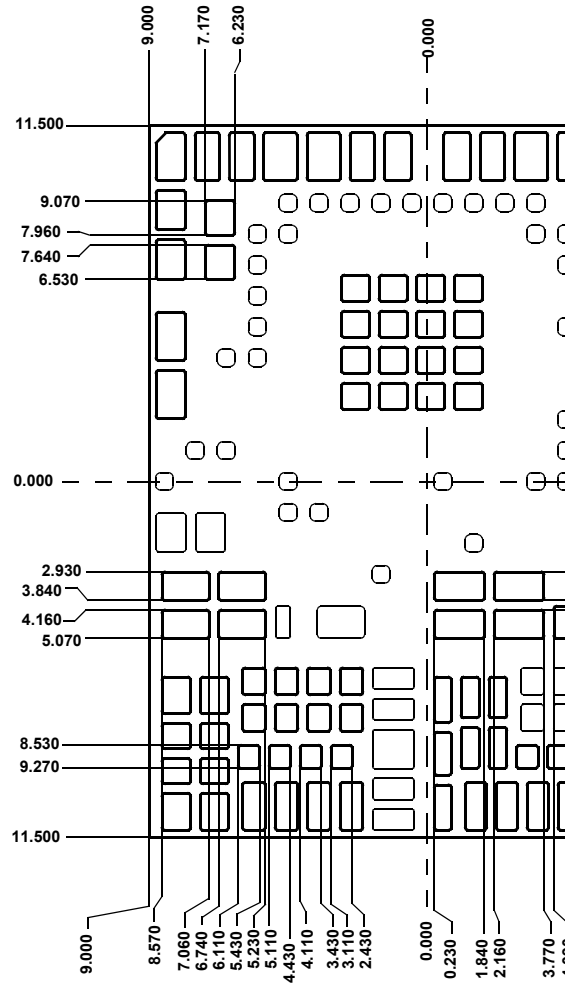
STENCIL OPENING EDGE POSITION
