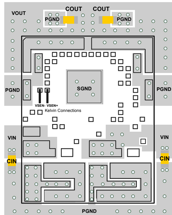
FIGURE 27. RECOMMENDED LAYOUT
