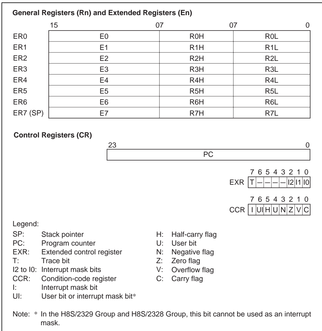
Figure 2.4 CPU Registers
