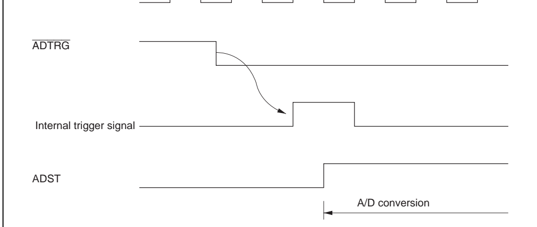
Figure 16.6 External Trigger Input Timing
