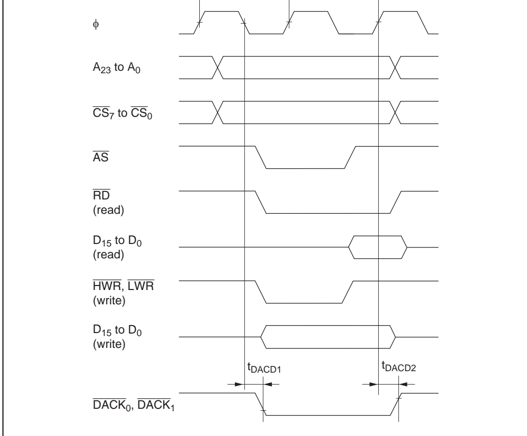
Figure 22.16 DMAC Single Address Transfer Timing (2-State Access)
