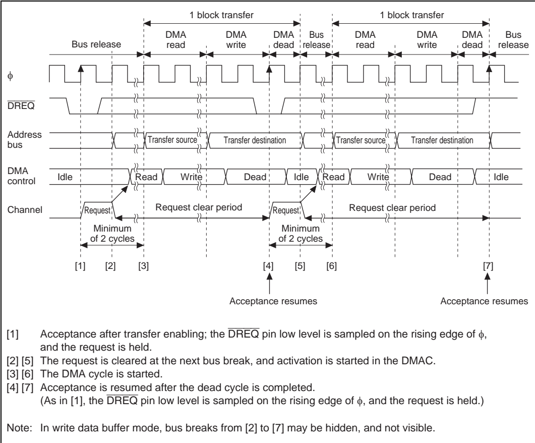
Figure 7.26 Example of \overline{DREQ} Level Activated Block Transfer Mode Transfer
