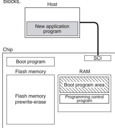
Figure 19.61 Boot Mode
