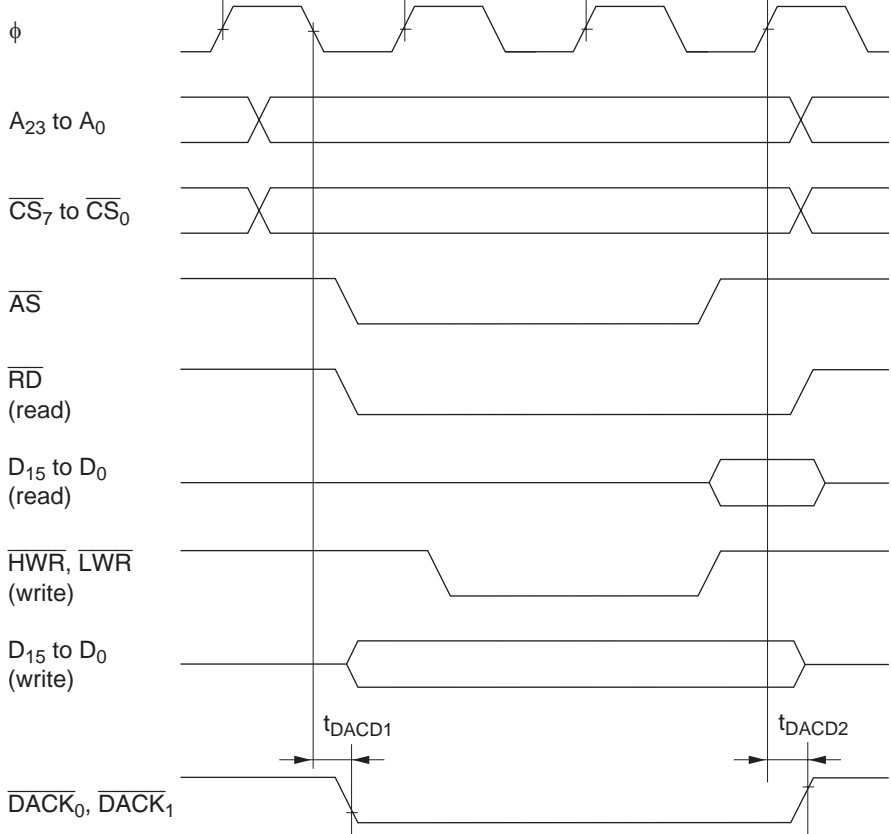
Figure 22.17 DMAC Single Address Transfer Timing (3-State Access)
