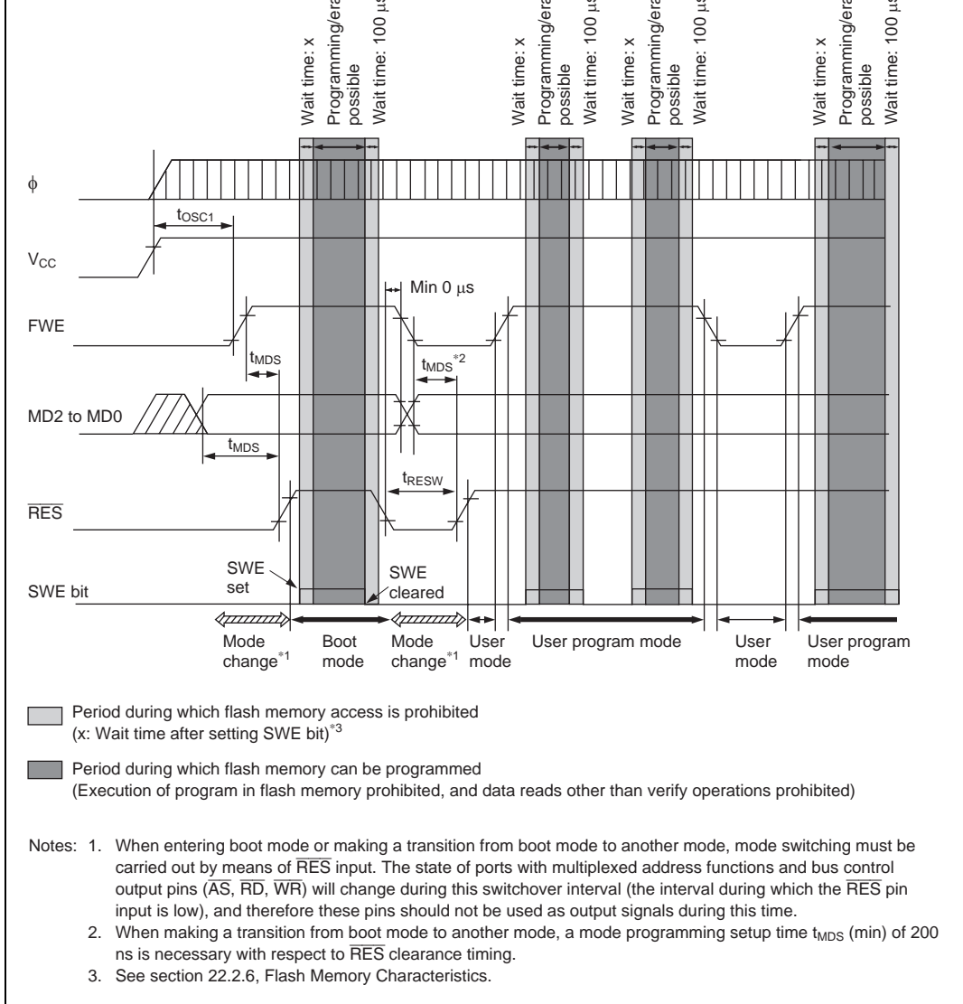
Figure 19.88 Mode Transition Timing (Example: Boot Mode → User Mode ↔ User Program Mode)
