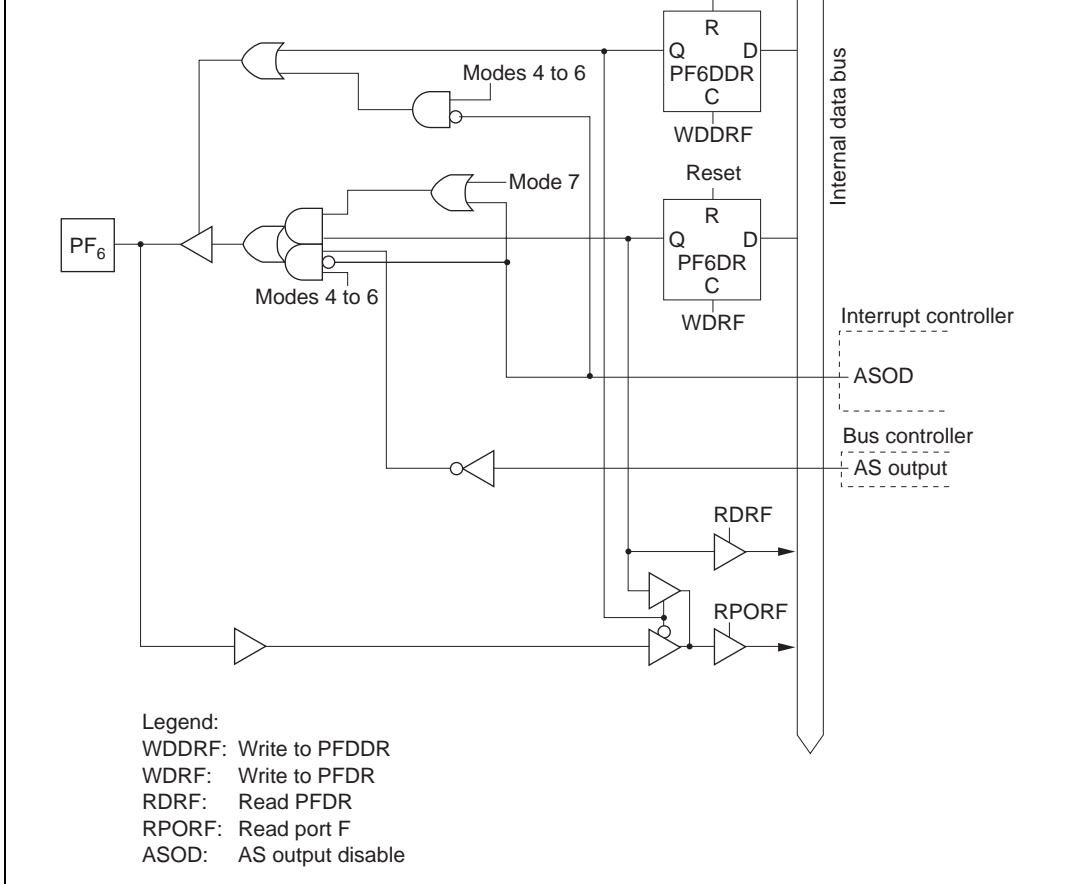
Figure C.12 (g) Port F Block Diagram (Pin PF 6 )
