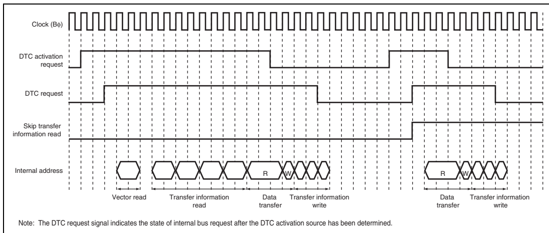
Figure 8.5 Transfer Information Read Skip Timing (Activated by On-Chip Peripheral Module; I \phi : B \phi : P \phi =1: 1/2: 1/2; Data Transferred from On-Chip Peripheral Module to On-Chip RAM; Transfer Information Is Written in 3 States)
