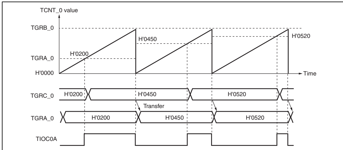
Figure 11.19 Example of Buffer Operation When TCNT_0 Clearing Is Selected for TGRB_0 to TGRA_0 Transfer Timing
