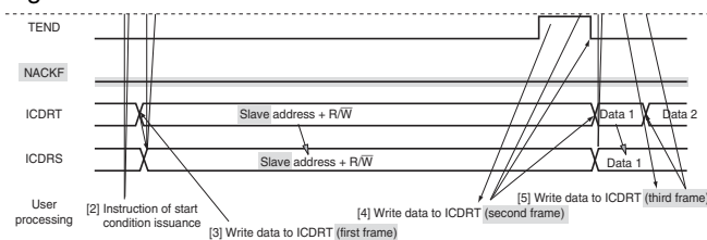
Figure 18.5 Master Transmit Mode Operation Timing (1)
