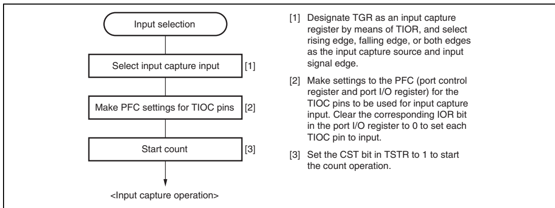
Figure 11.10 Example of Input Capture Operation Setting Procedure
