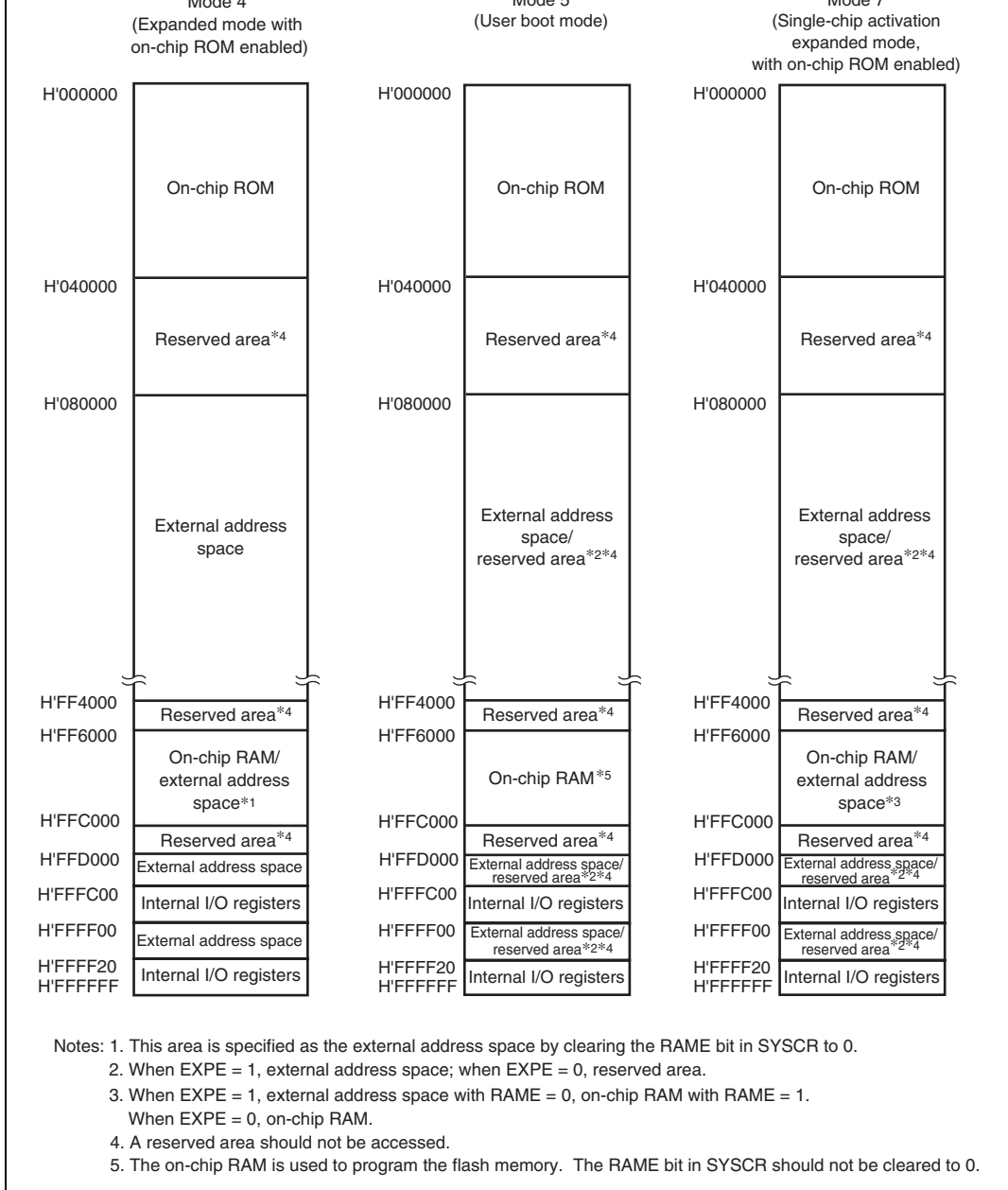
Figure 3.10 H8S/2361F Memory Map (2)
