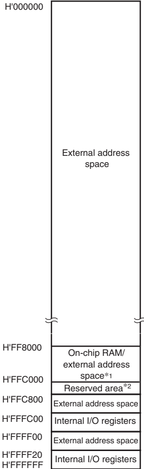
Figure 3.15 H8S/2363 Memory Map
