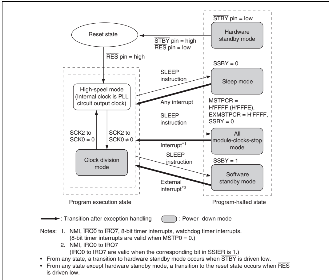
Figure 23.1 Mode Transitions
