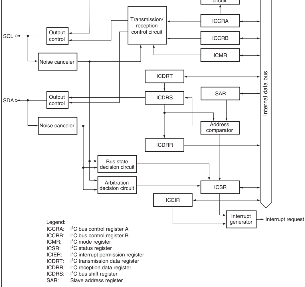
Figure 15.1 Block Diagram of I 2 C Bus Interface2
