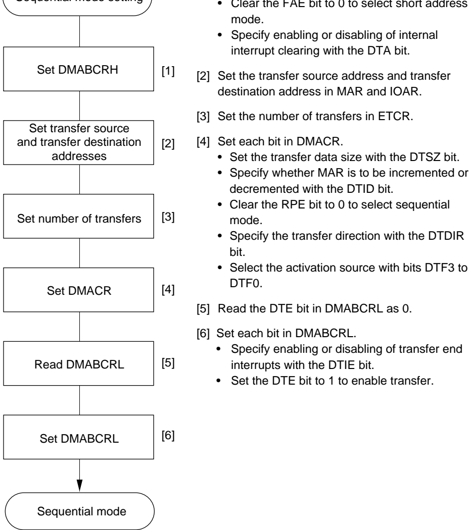
Figure 7.4 Example of Sequential Mode Setting Procedure
