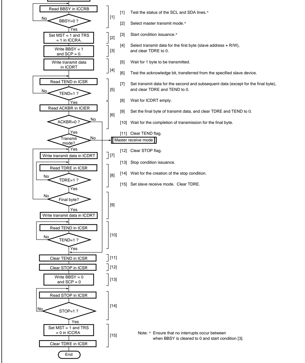
Figure 15.14 Sample Flowchart for Master Transmit Mode
