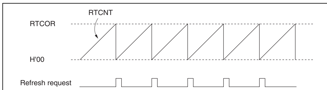
Figure 7.25 RTCNT Operation
