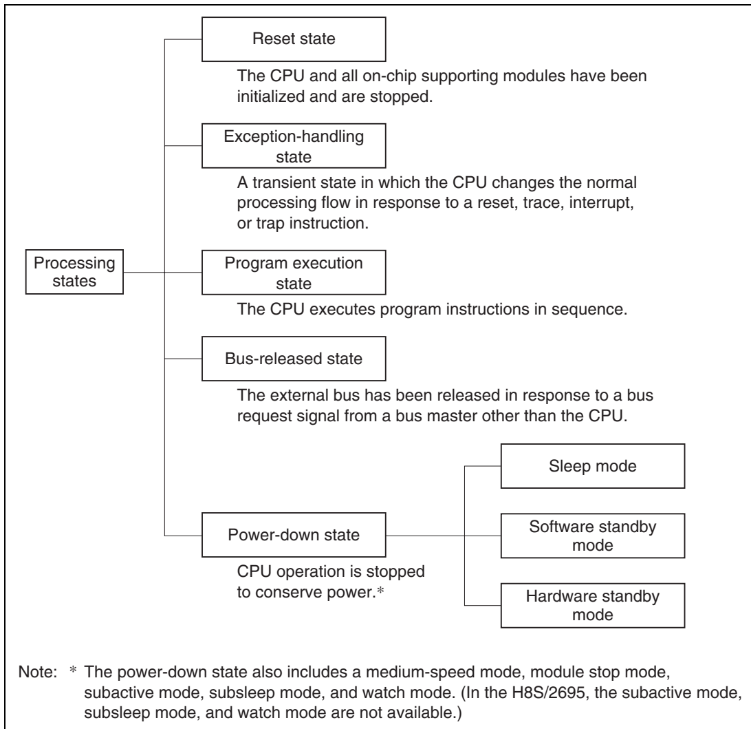
Figure 2.14 Processing States
