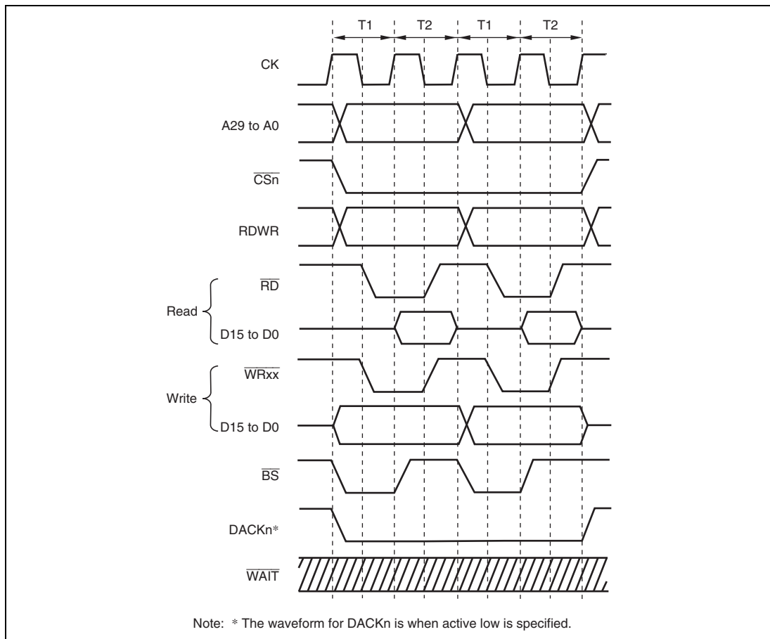
Figure 9.4 Continuous Access for Normal Space 2 Bus Width = 16 Bits, Longword Access, WM Bit in CSnWCR = 1 (Access Wait = 0, Cycle Wait = 0)
