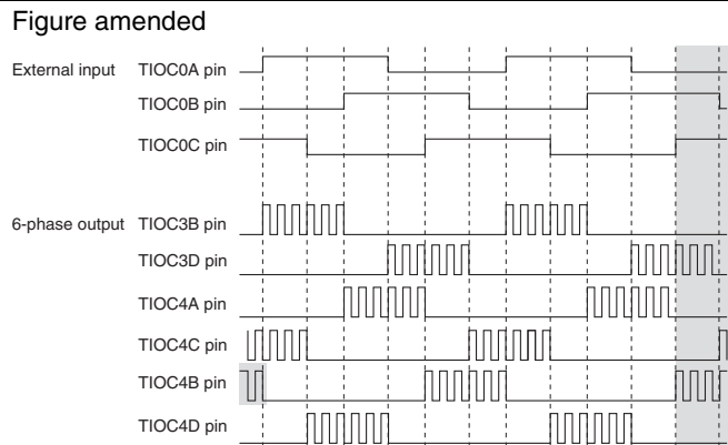
Figure 11.70 Example of Output Phase Switching by External Input (2)
