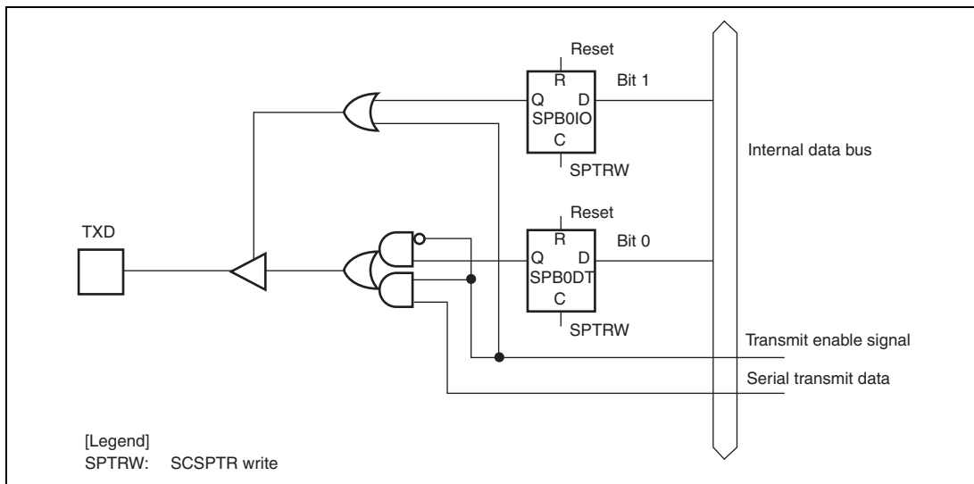
Figure 15.20 SPB0IO Bit, SPB0DT bit, and TXD Pin
