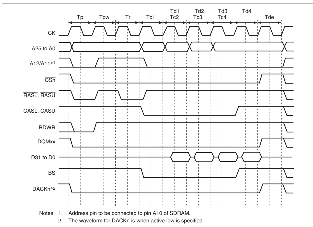
Figure 9.25 Burst Read Timing (Bank Active, Different Row Addresses)
