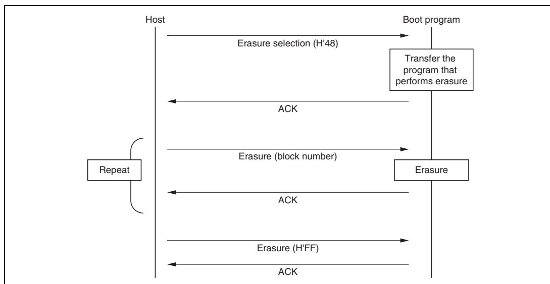
Figure 23.27 Sequence of Erasure
