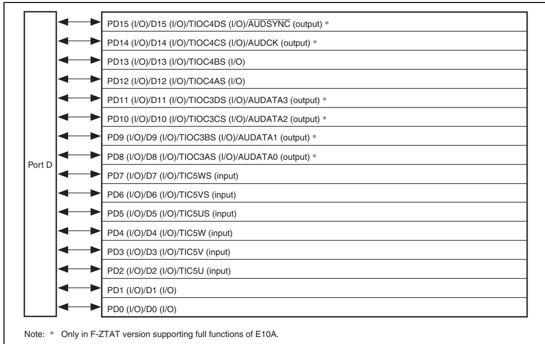
Figure 22.9 Port D (SH7083, SH7084)
