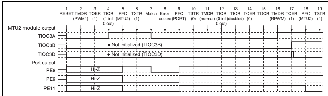
Figure 11.152 Error Occurrence in PWM Mode 1, Recovery in Reset-Synchronized PWM Mode
