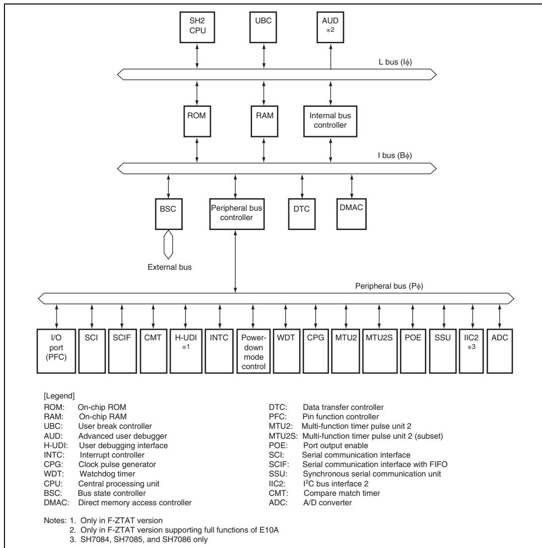
Figure 1.1 Block Diagram
