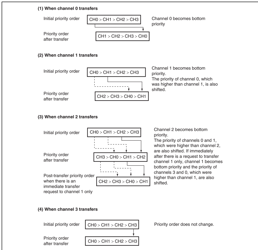
Figure 10.3 Round-Robin Mode
