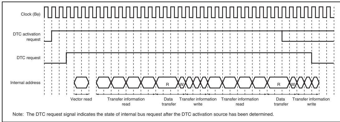
Figure 8.12 Example of DTC Operation Timing: Chain Transfer (Activated by On-Chip Peripheral Module; Iφ: Bφ: Pφ =1: 1/2: 1/2; Data Transferred from On-Chip Peripheral Module to On-Chip RAM; Transfer Information Is Written in 3 Cycles)
