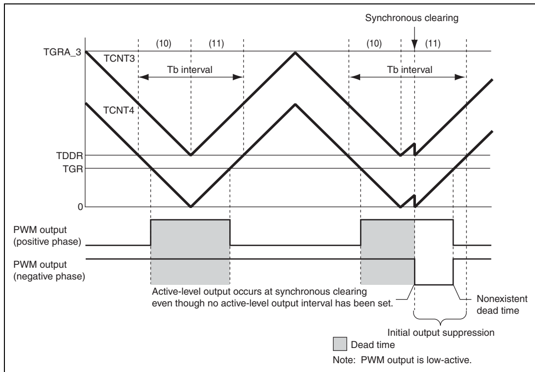
Figure 11.138 Condition (2) Synchronous Clearing Example
