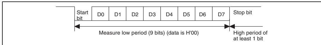
Figure 23.7 Automatic Adjustment Operation of SCI Bit Rate
