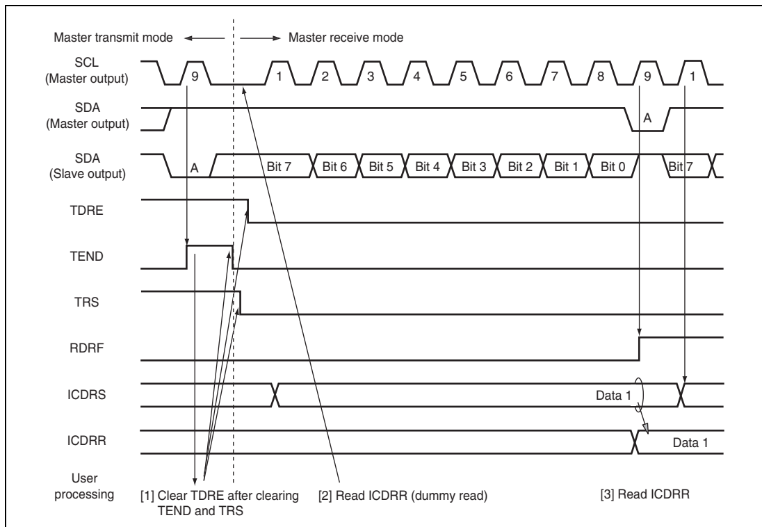
Figure 18.8 Master Receive Mode Operation Timing (1)
