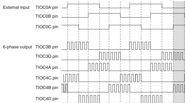
Figure 11.70 Example of Output Phase Switching by External Input (2)
