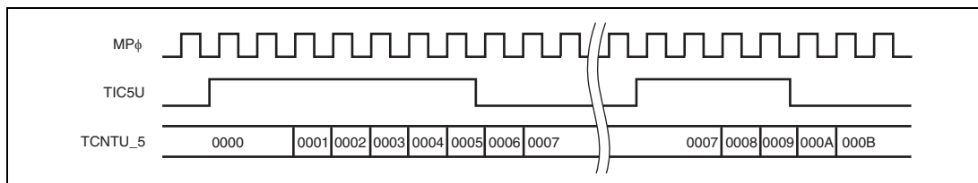
Figure 11.88 Example of External Pulse Width Measurement (Measuring High Pulse Width)
