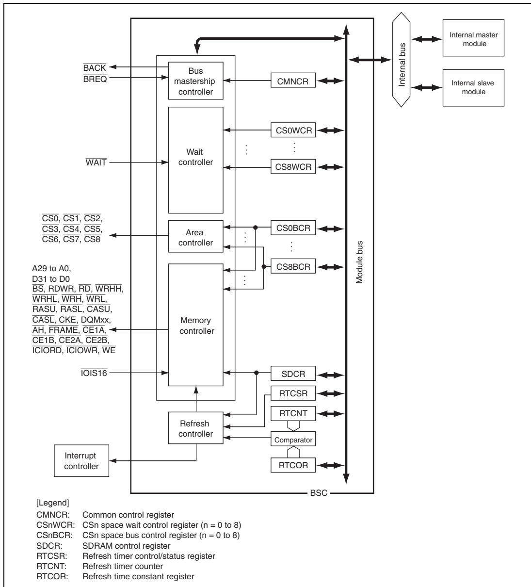
Figure 9.1 Block Diagram of BSC
