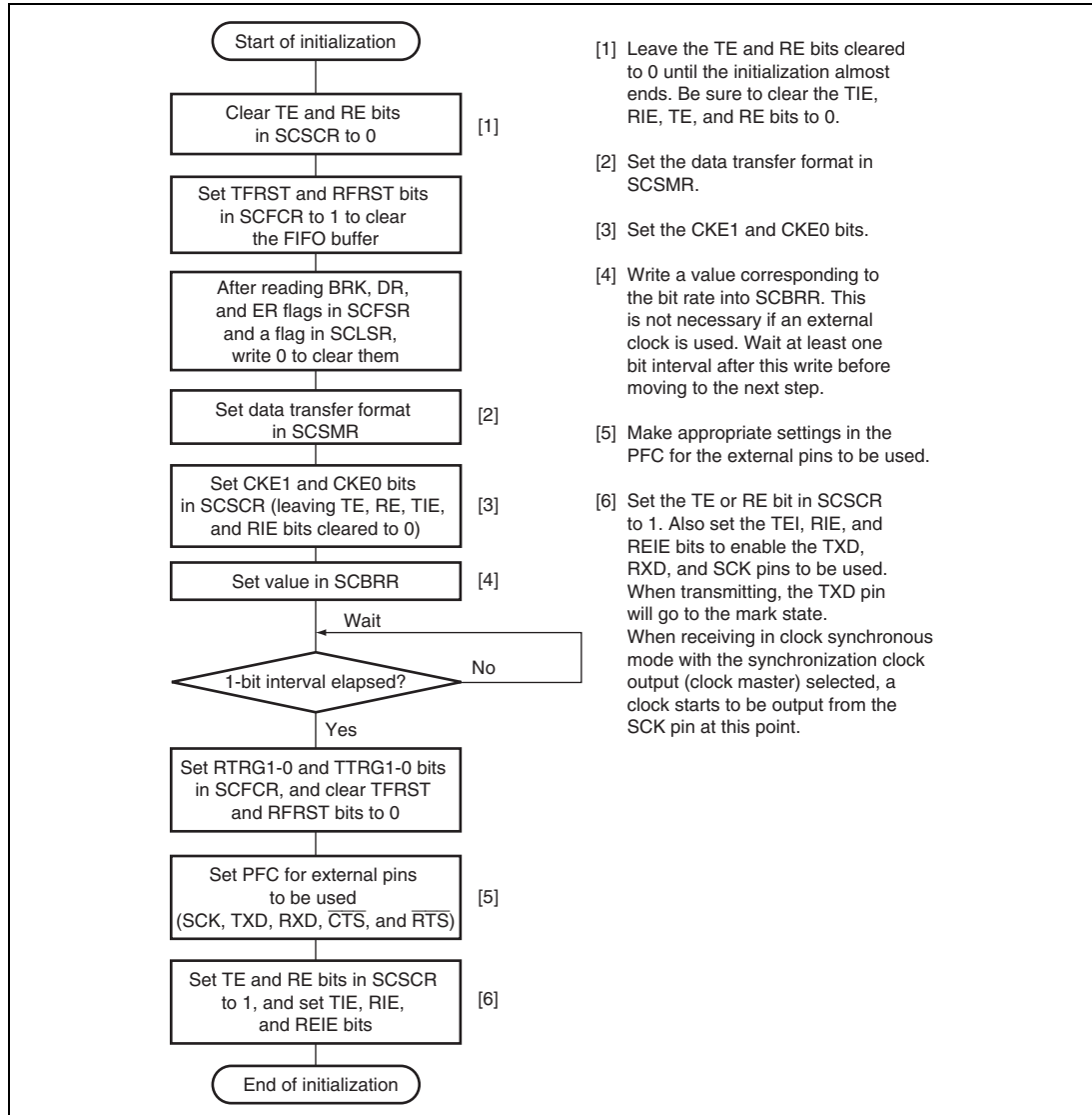
Figure 16.12 Sample Flowchart for SCIF Initialization
