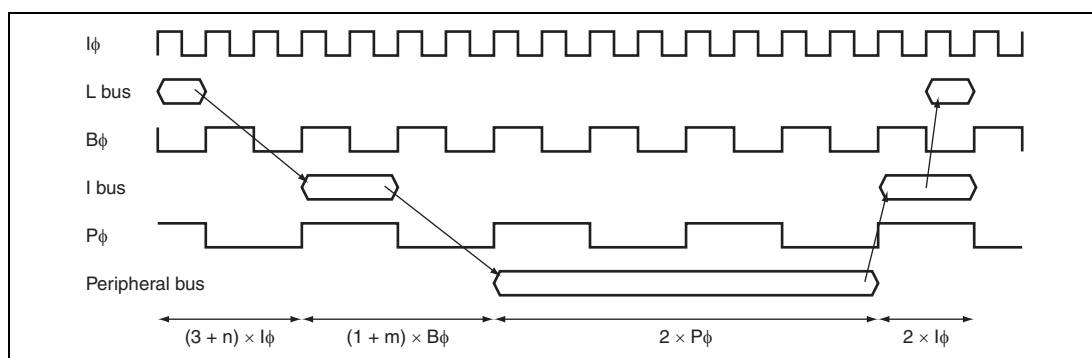
Figure 9.54 Timing of Read Access to On-Chip Peripheral I/O Registers When I\phi:B\phi:P\phi = 4:2:1
