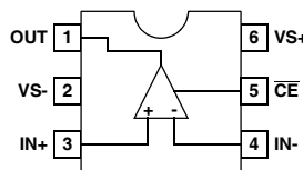
EL5192A (6 LD SOT-23) TOP VIEW
