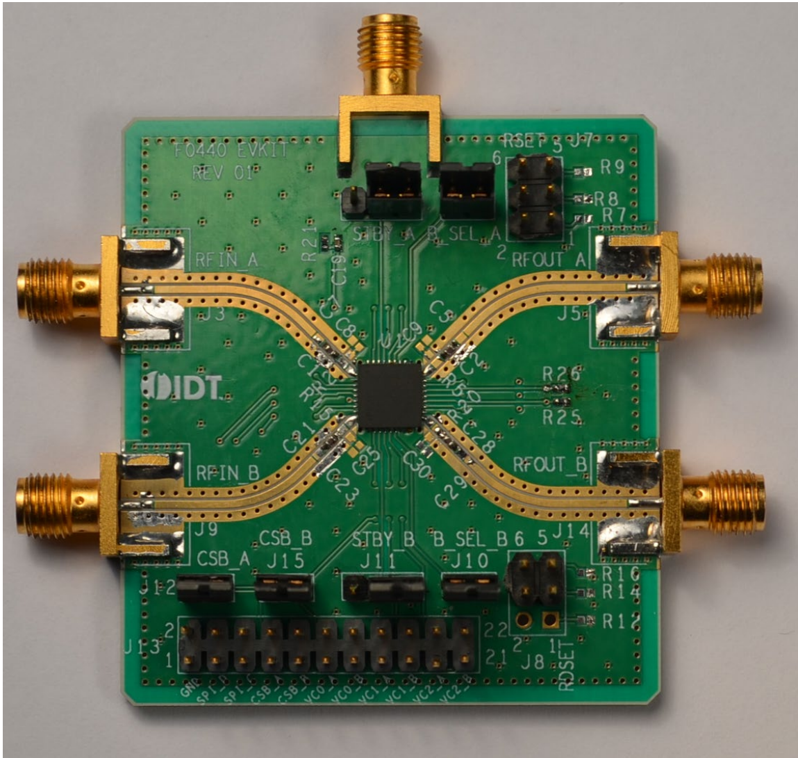
Figure 42. Top View
