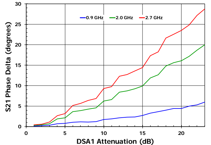
Figure 24. Phase Change as DSA1 varied [DSA0=0dB, DSA2=0dB]
