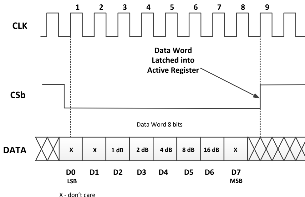
Figure 41. Serial Register Timing Diagram (LSB-FIRST)
