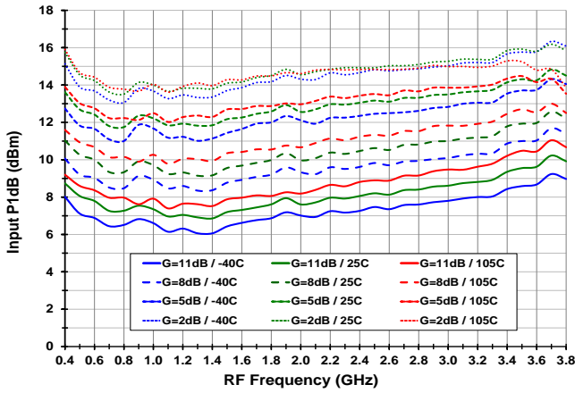
Figure 9. Input P1dB vs. Temperature and Gain Setting
