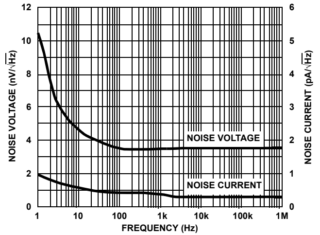
FIGURE 6. NOISE CHARACTERISTICS
