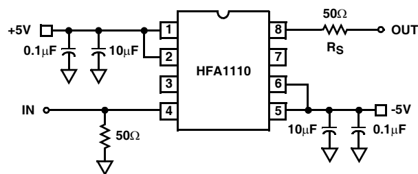
SCHEMATIC DIAGRAM
