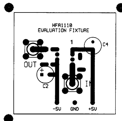
TOP LAYOUT
