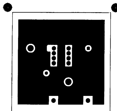
TOP LAYOUT
