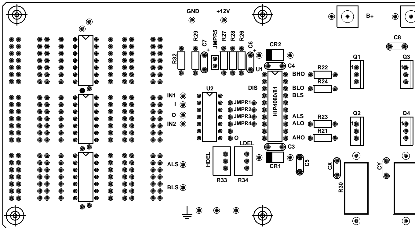
FIGURE 32. HIP4081A EVALUATION BOARD SILKSCREEN
