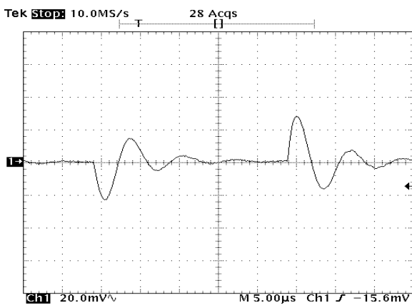
FIGURE 24. LINE TRANSIENT RESPONSE, 0.001\mu F LOAD CAPACITANCE
